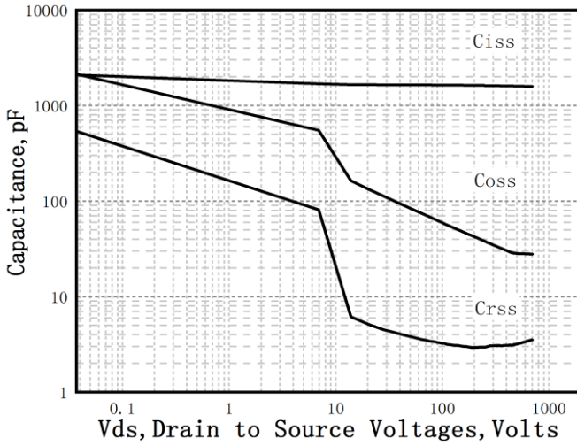
Figure 7. Capacitance Characteristics
