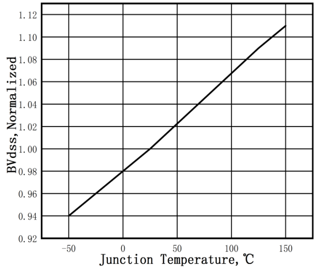
Figure 6. Normalized BV_{DS} vs. Temperature
