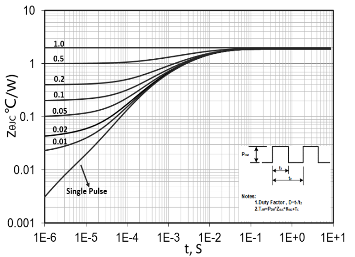
Figure 10. Transient Thermal Response Curve (TO-220F)
